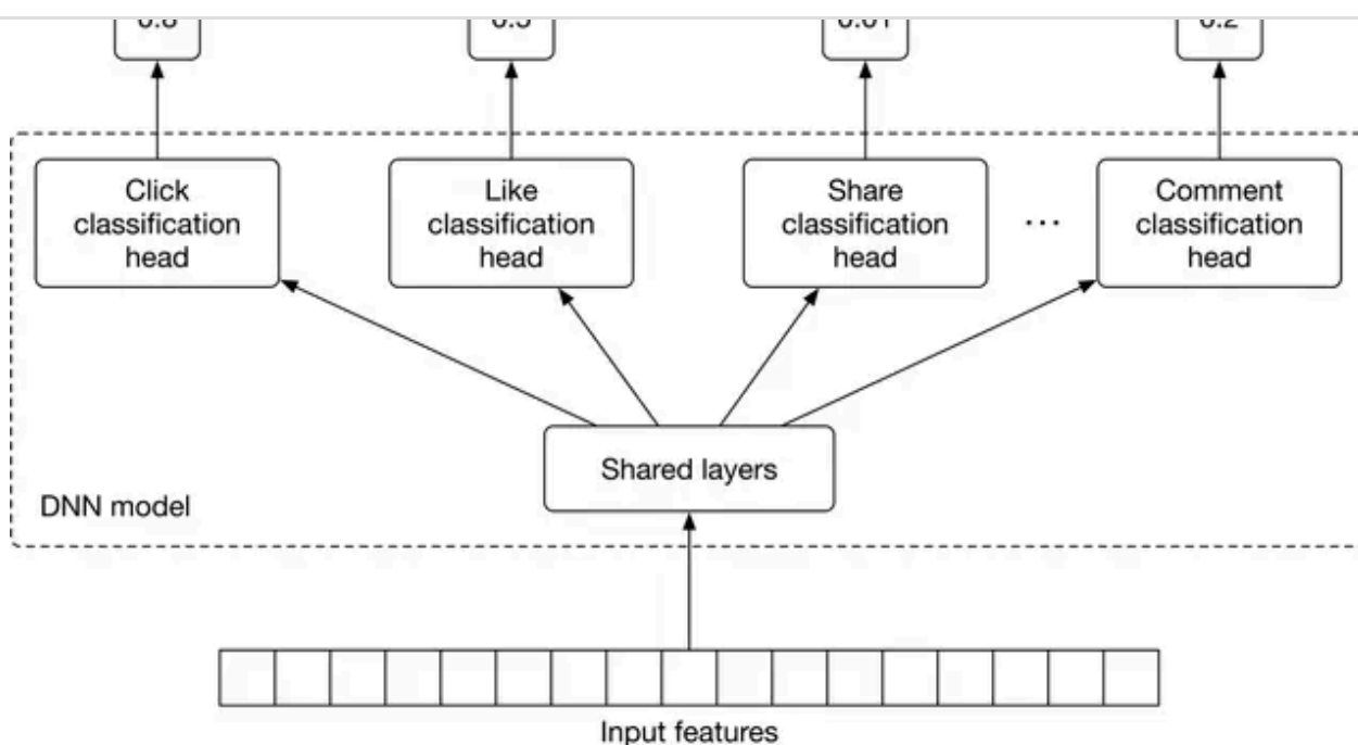
Figure 10.9: Multi-task DNN
