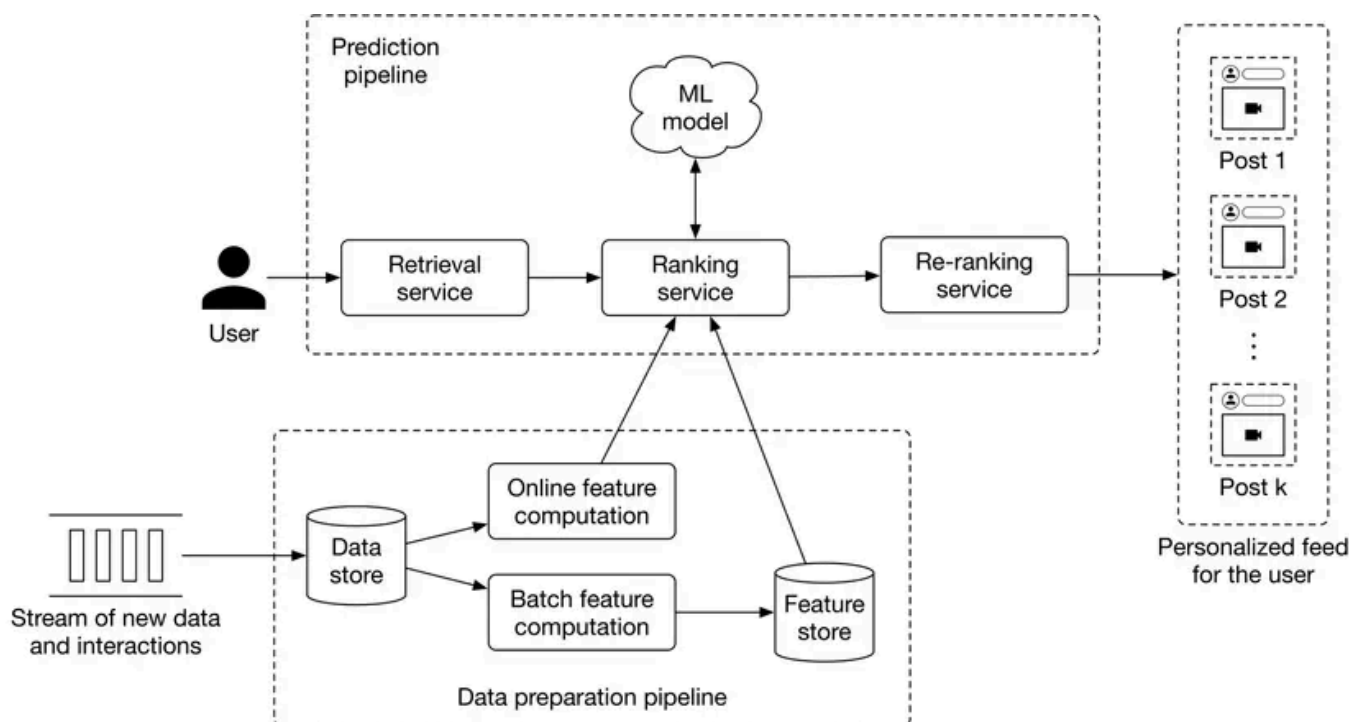
Figure 10.14: ML system design of a personalized news feed system
