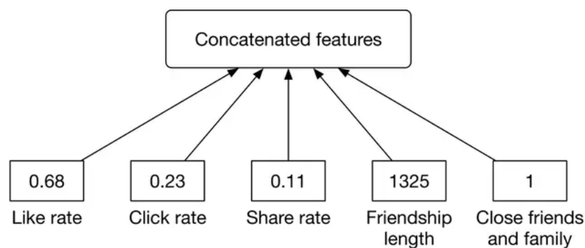
Figure 10.7: User-author affinity features
